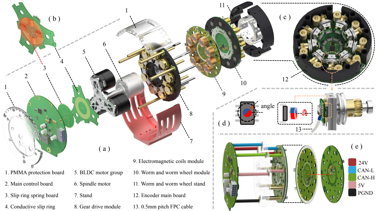
Fig. 2. Drive box structure. (a) Exploded view of the drive box. (b) Slip ring structure. (c) Structure of the magnetic encoder groups. (d) Schematic and structure of the encoder. (e) Pathway for power and data transmission.
